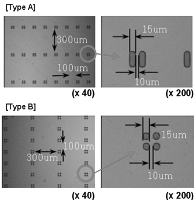
FIGURE 2 The photographs of designed micro-structure of columnar spacer array. Circled insets in left figures are magnified at the right by 5 times ( \times 40 to \times 200 ).
