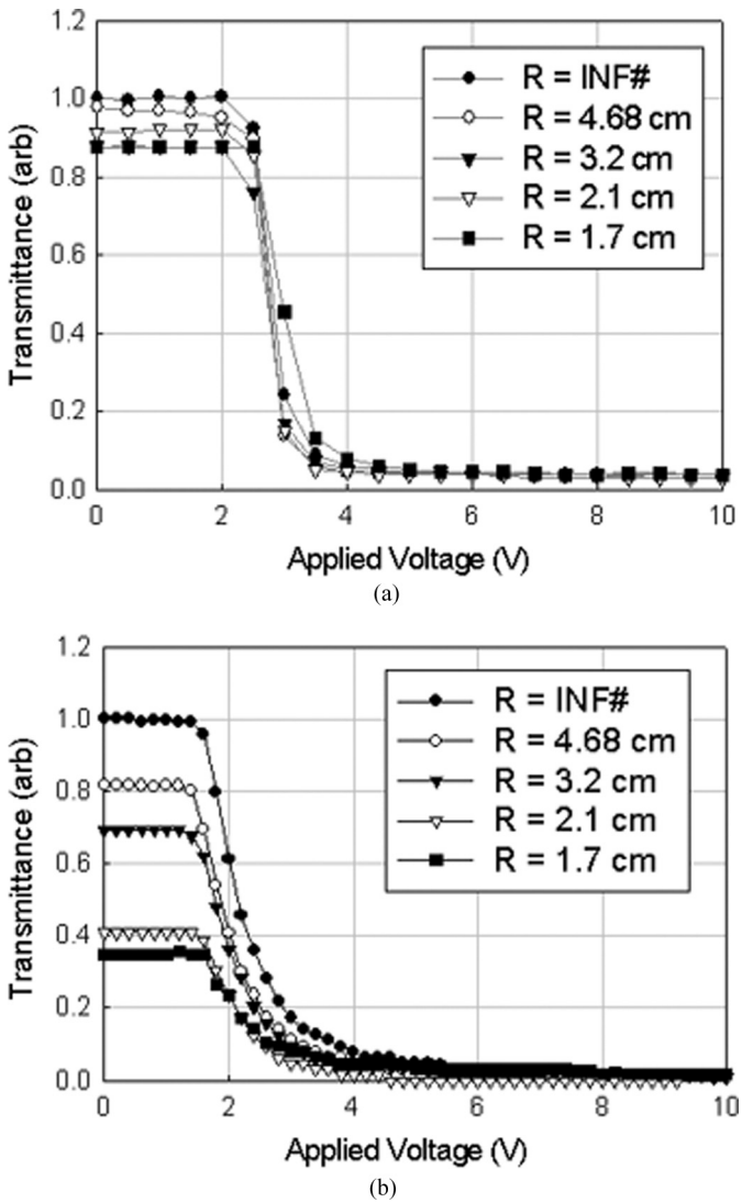
FIGURE 4 Electro-optic characteristics of the sample under various external deformations. (a) Voltage-Transmittance curve of flexible display ECB mode sample with micro-structure and \mu CP assembling technique. (b) V-T curve of conventional ECB sample with plastic substrate and ball spacer only.
